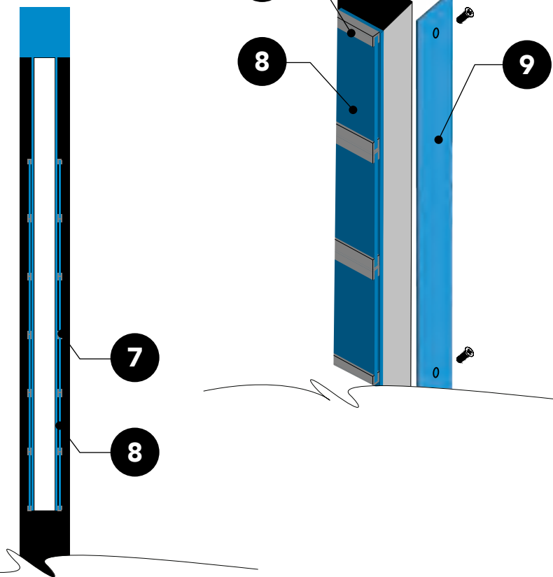
Side View Scale 1 1/2"=1'
